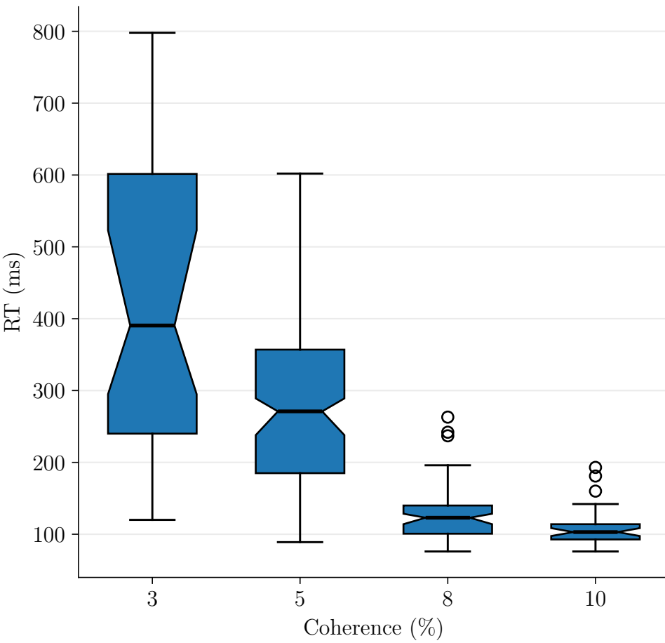
RT Distributions at Low Coherence Levels
